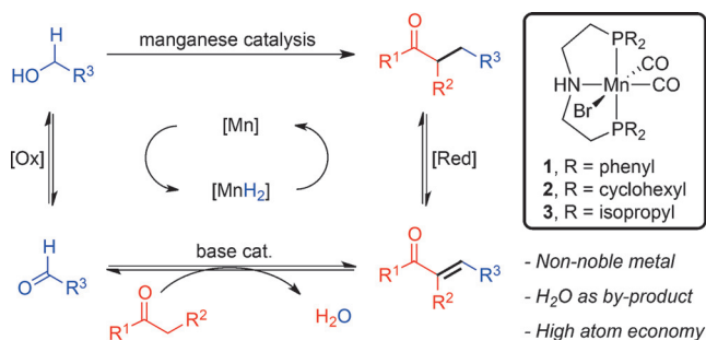
Scheme 1. Manganese-catalyzed \alpha -alkylation of ketones with alcohols.
